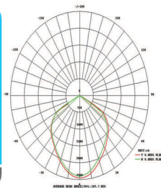
Distribution curve
