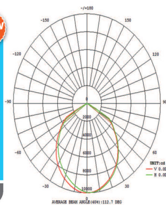
Distribution curve
